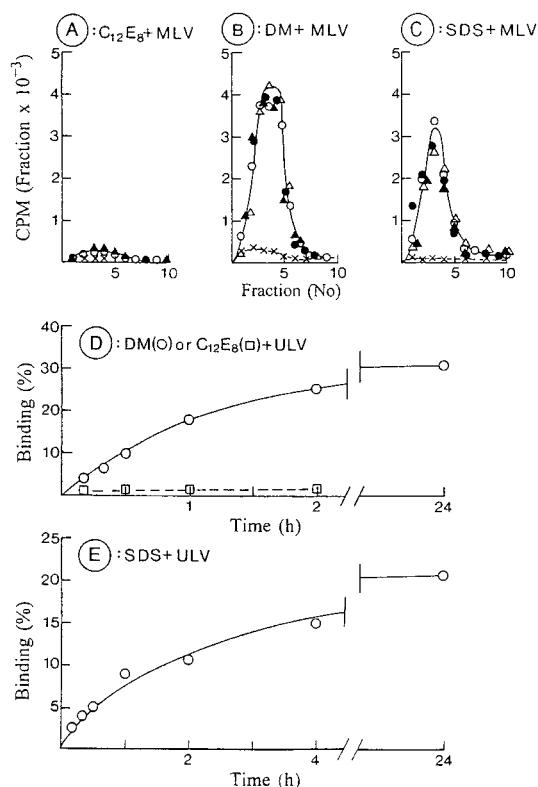
FIGURE 8 Detergent release from DOPC multilayers and uptake by DOPC unilamellar liposomes at 20°C. ( Upper figures, A, B, and C ) To examine detergent release C_{12}E_8 (A), dodecylmaltoside (B) or SDS (C) was encapsulated in a DOPC liposome preparation (at 5 mg/ml) during the formation of multilayered vesicles (MLVs) by vortexing thin DOPC films in 10 mM TES (pH 7.4), 100 mM NaCl, and 0.1 mM CaCl_2 , containing 0.4 mg/ml of detergent with radioactive tracer. At the start of the experiment (zero time), a sample was diluted 100 times with detergent-free buffer, and 2.5-ml aliquots of this dilution (containing 12,000–13,000 cpm) were applied to a Biobeads column (1 \times 5 cm) immediately after dilution (○) and at different times thereafter: ●, 15 min; △, 30 min; and ▲, 5 h. x—x, shows the elution from control samples, without phospholipid, treated the same way to indicate the completeness of detergent extraction from the buffer by passage through the column. ( Middle and lower figures, D and E ) To examine detergent uptake by liposomal membranes, radiolabeled and unlabeled detergent (0.4 mg/ml) was added at time 0 to unilamellar vesicles (ULVs) of DOPC liposomes (5 mg/ml), prepared by cholate dialysis, and suspended in 10 mM TES (pH 7.4), 100 mM NaCl, and 0.1 mM CaCl_2 at time 0. At various times thereafter, aliquots of the samples were diluted 100 times with detergent-free buffer, and 2.5 ml of these dilutions (containing 12,000–13,000 cpm) was applied to the Biobeads column. Intravesicular uptake of dodecylmaltoside and SDS (○) was calculated from the radioactivity in the first eight fractions, with a subtraction of the zero time elution value (2–7%) to correct for the presence of detergent remaining in the medium and in the outer bilayer leaflet after passage through the column. Note that in the case of C_{12}E_8 (□), the apparent lack of uptake reflects the fact that the release is too fast to allow retention by the liposomes of detergent taken up during the incubation period within the time scale (2 min) of the subsequent chromatography (cf. le Maire et al., 1987).
